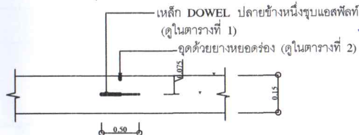
1 CONSTRUCTION JOINT
